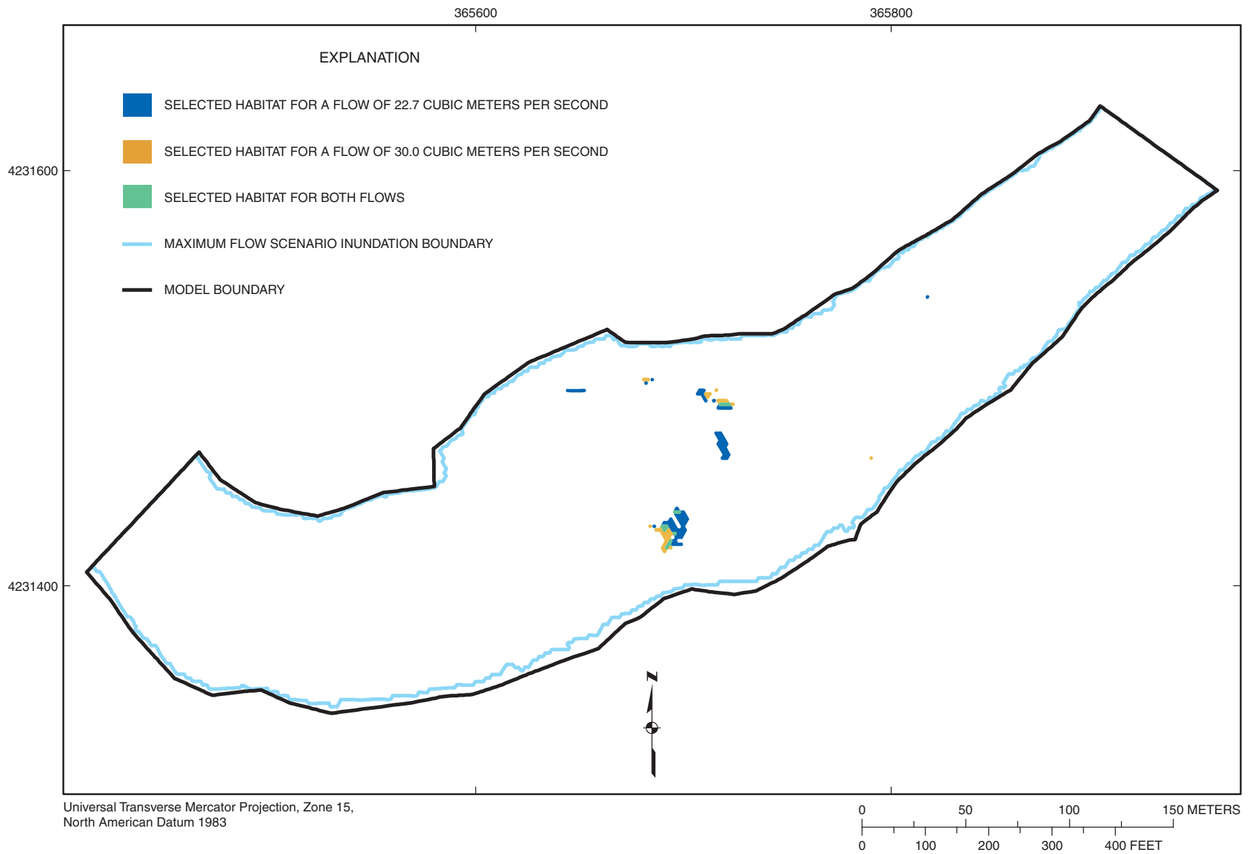
Figure 4-88. Selected habitat area distribution for habitat category 22 (channel catfish) at flows of 22.7 and 30.0 cubic meters per second at Marais des Cygnes River site MDC2.
